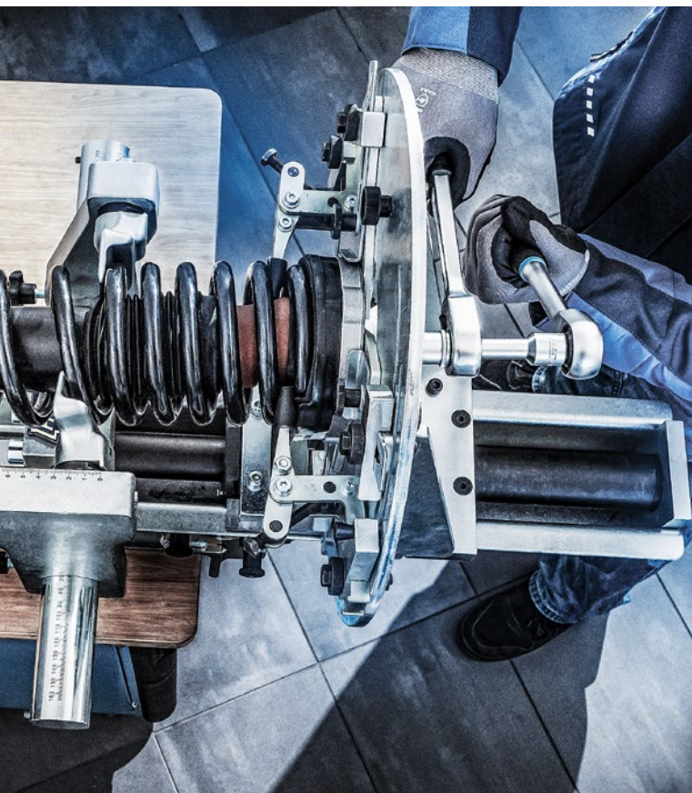
Spring strut fixation
