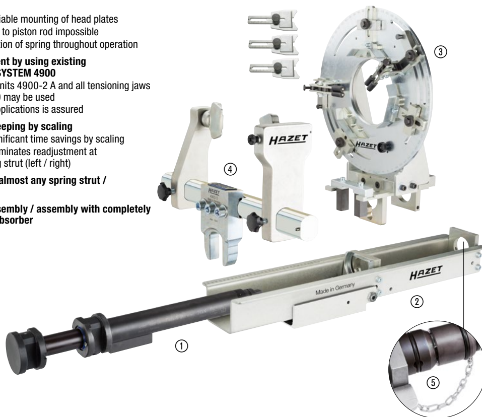
Safety spring vice 4903/4
